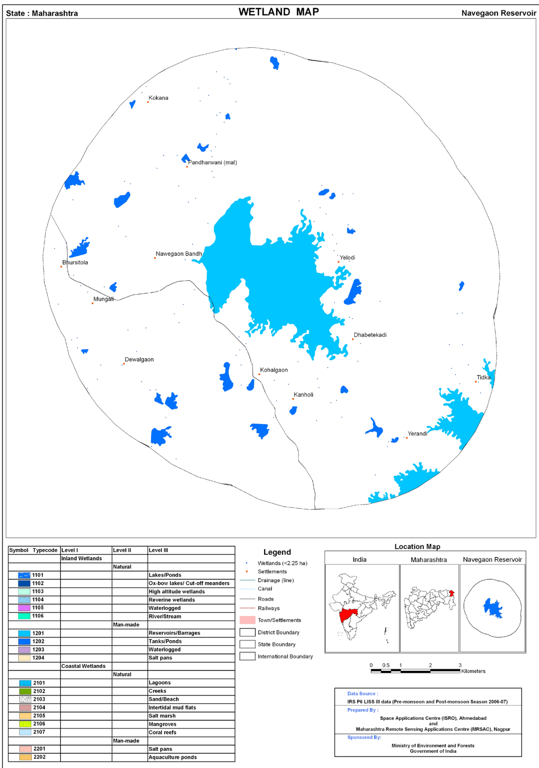
Plate 16: Wetland map - 5 km buffer area of Navegaon Notified Wetland
