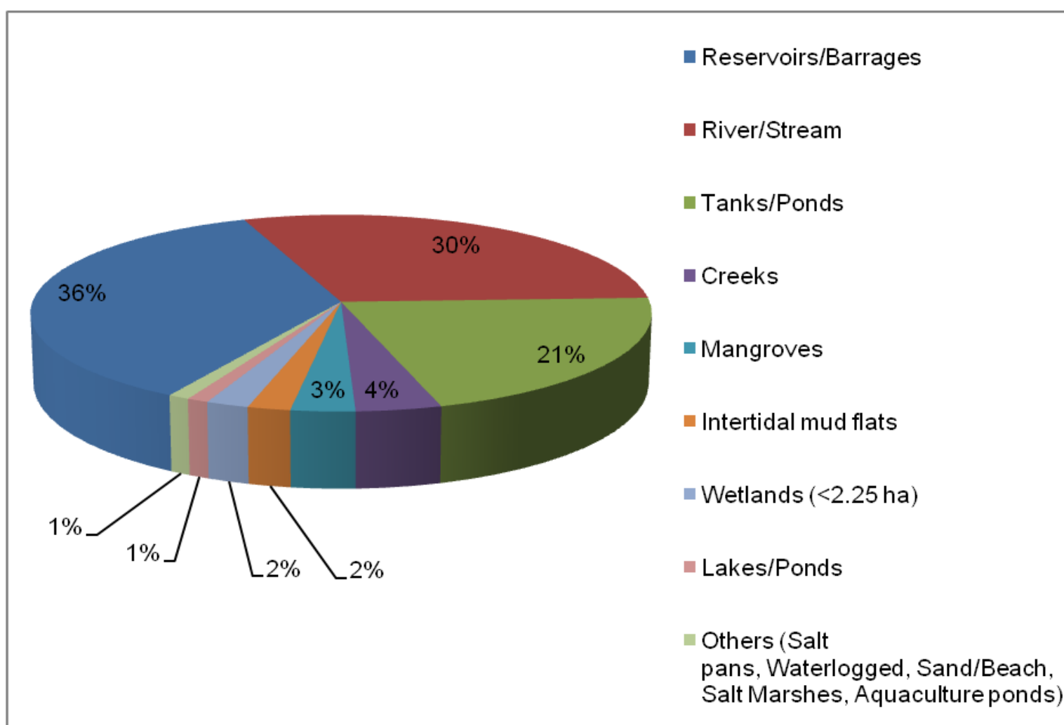
Figure 10: Type-wise wetland distribution in Maharashtra
