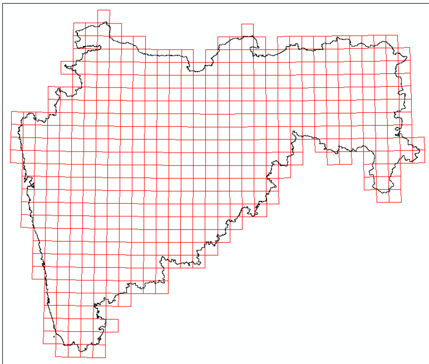
Figure 4: Spatial Framework of Maharashtra
