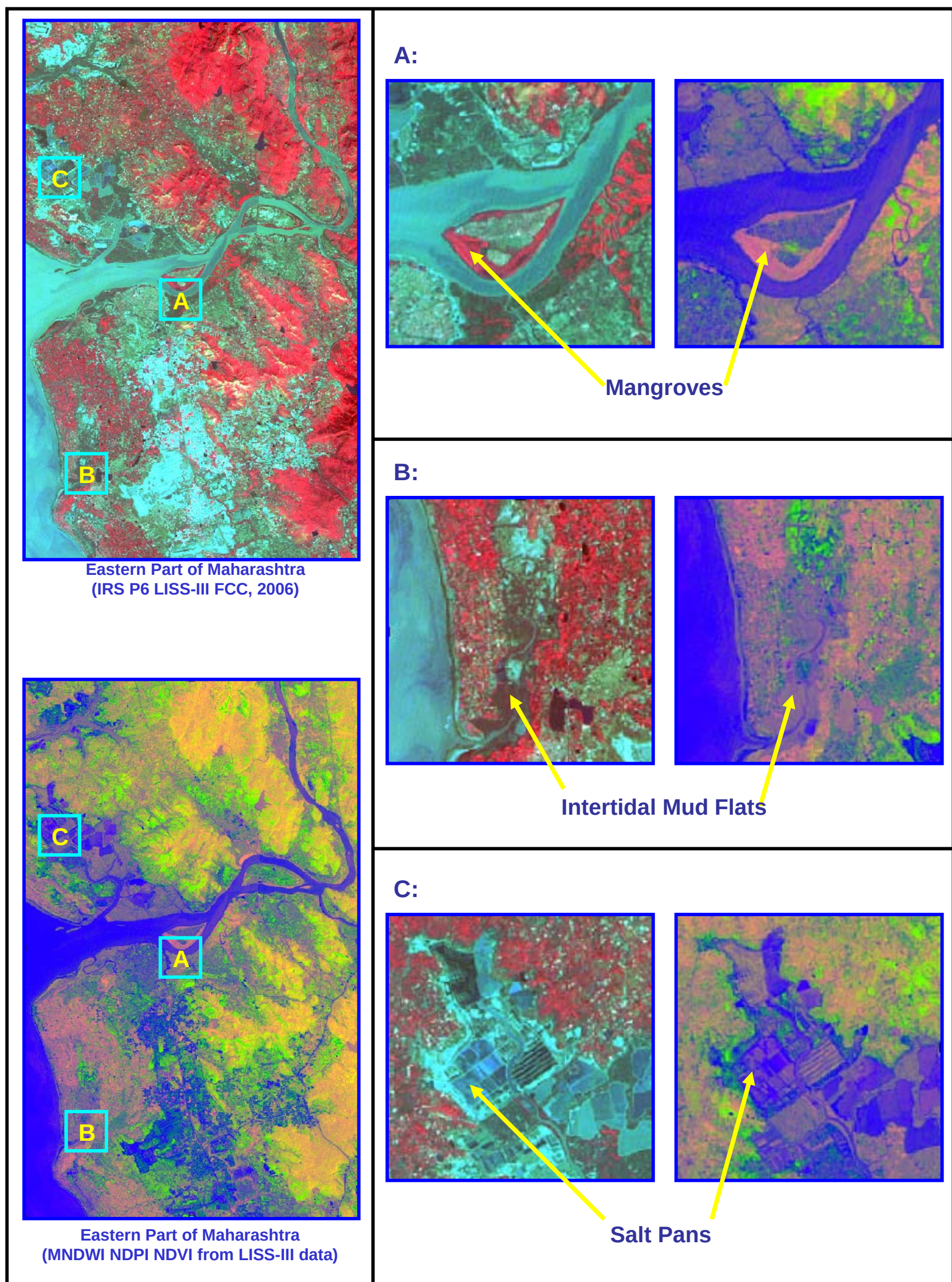
Plate – 1b: Major wetland types of Maharashtra as seen and deciphered from remote sensing data
