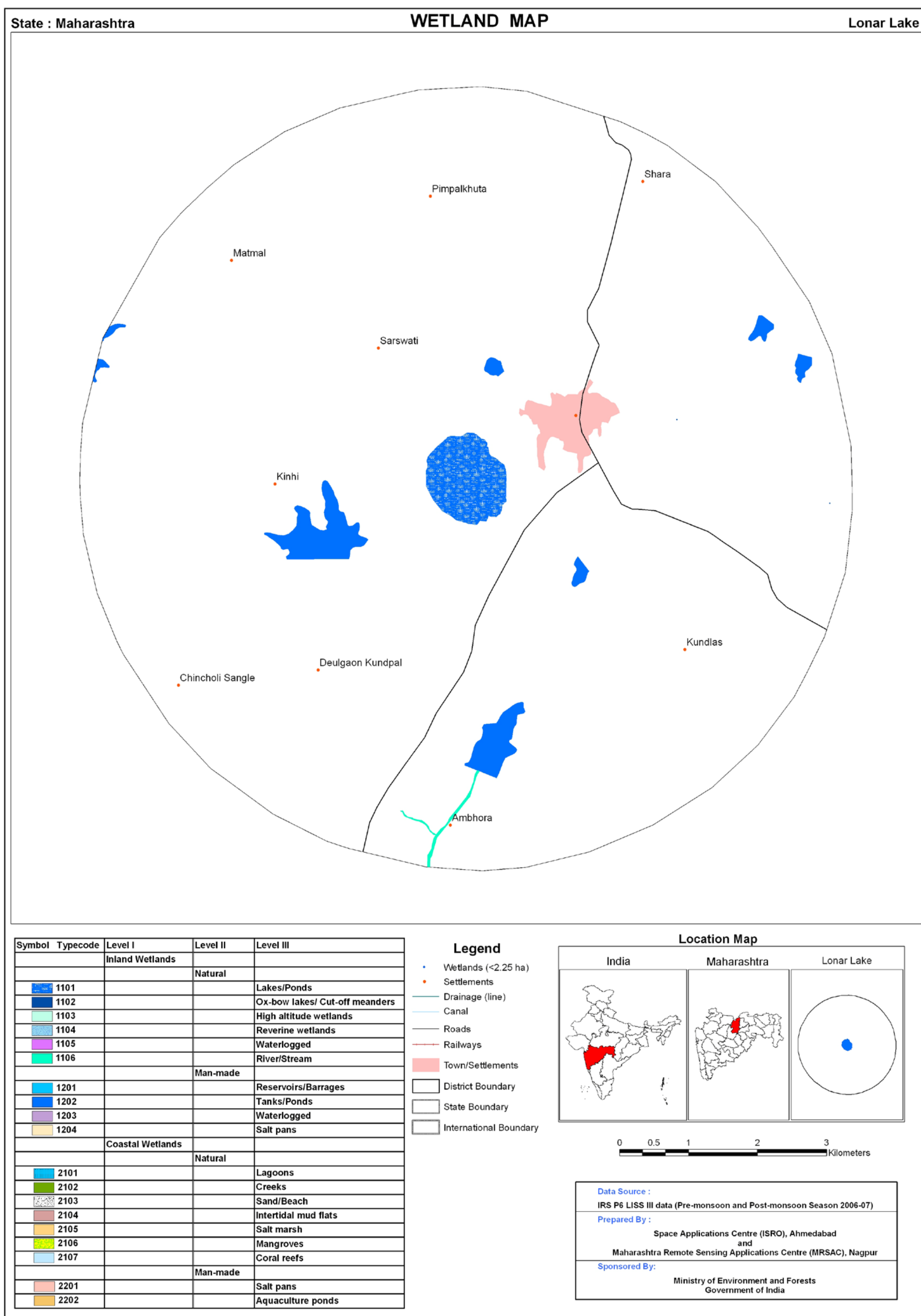
Plate 4: Wetland map - 5 km buffer area of Lonar Lake
