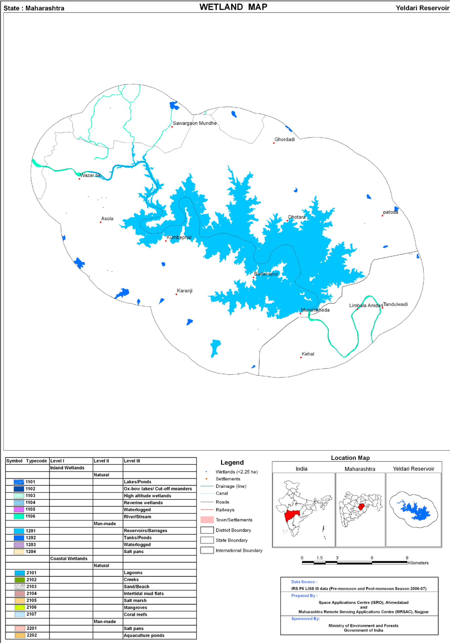
Plate 10: Wetland map - 5 km buffer area of Yeldari Reservoir
