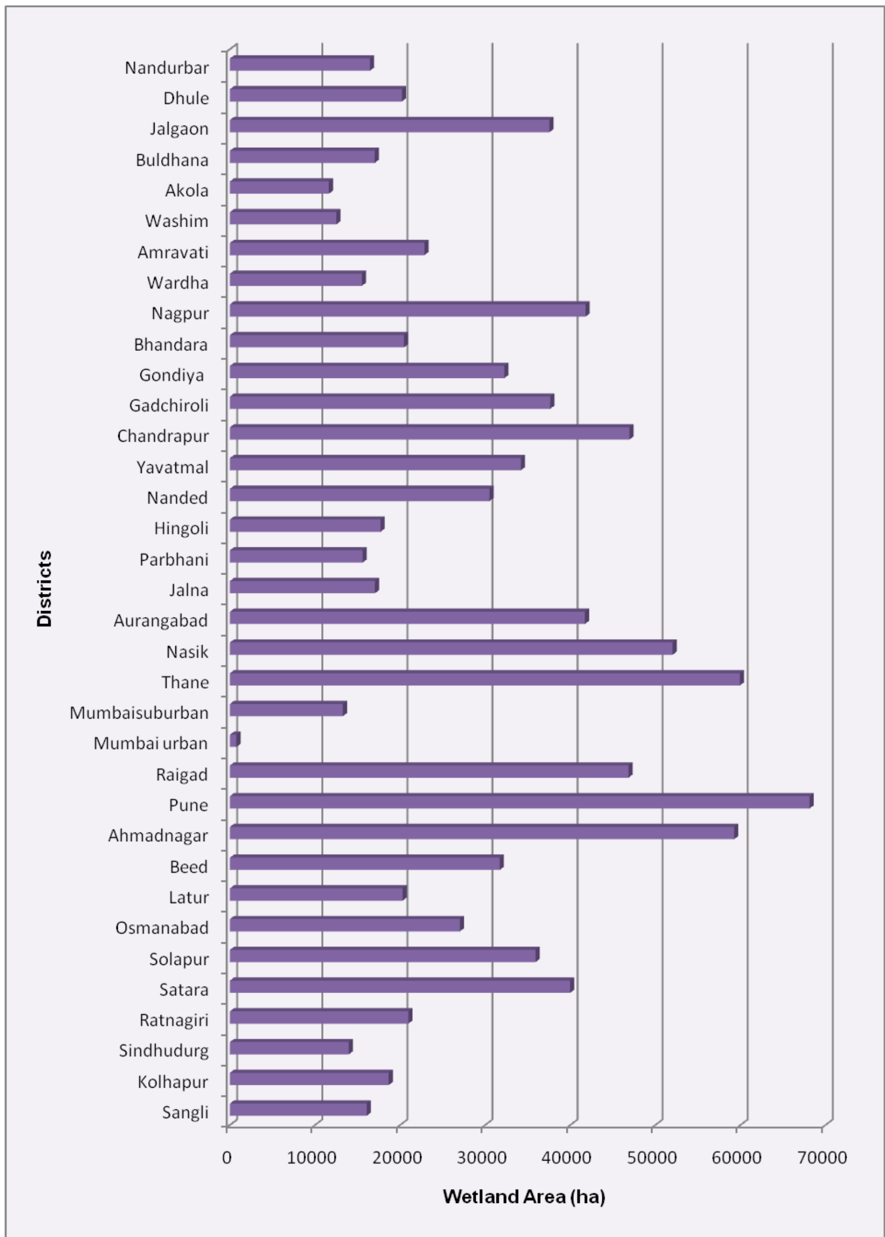
Figure 11: District-wise graphical distribution of wetlands
