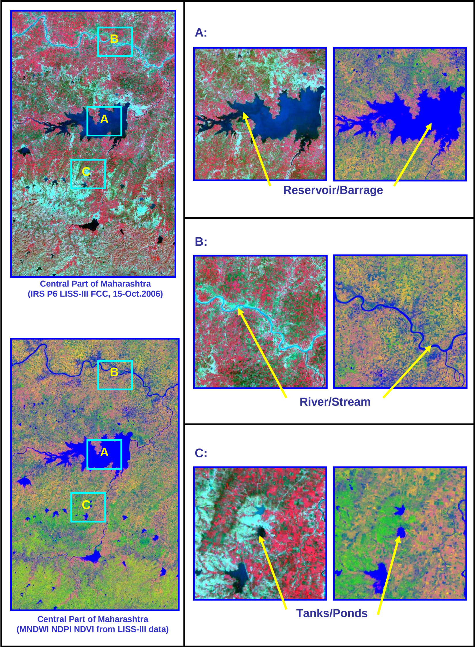
Plate – 1a: Major wetland types of Maharashtra as seen and deciphered from remote sensing data
