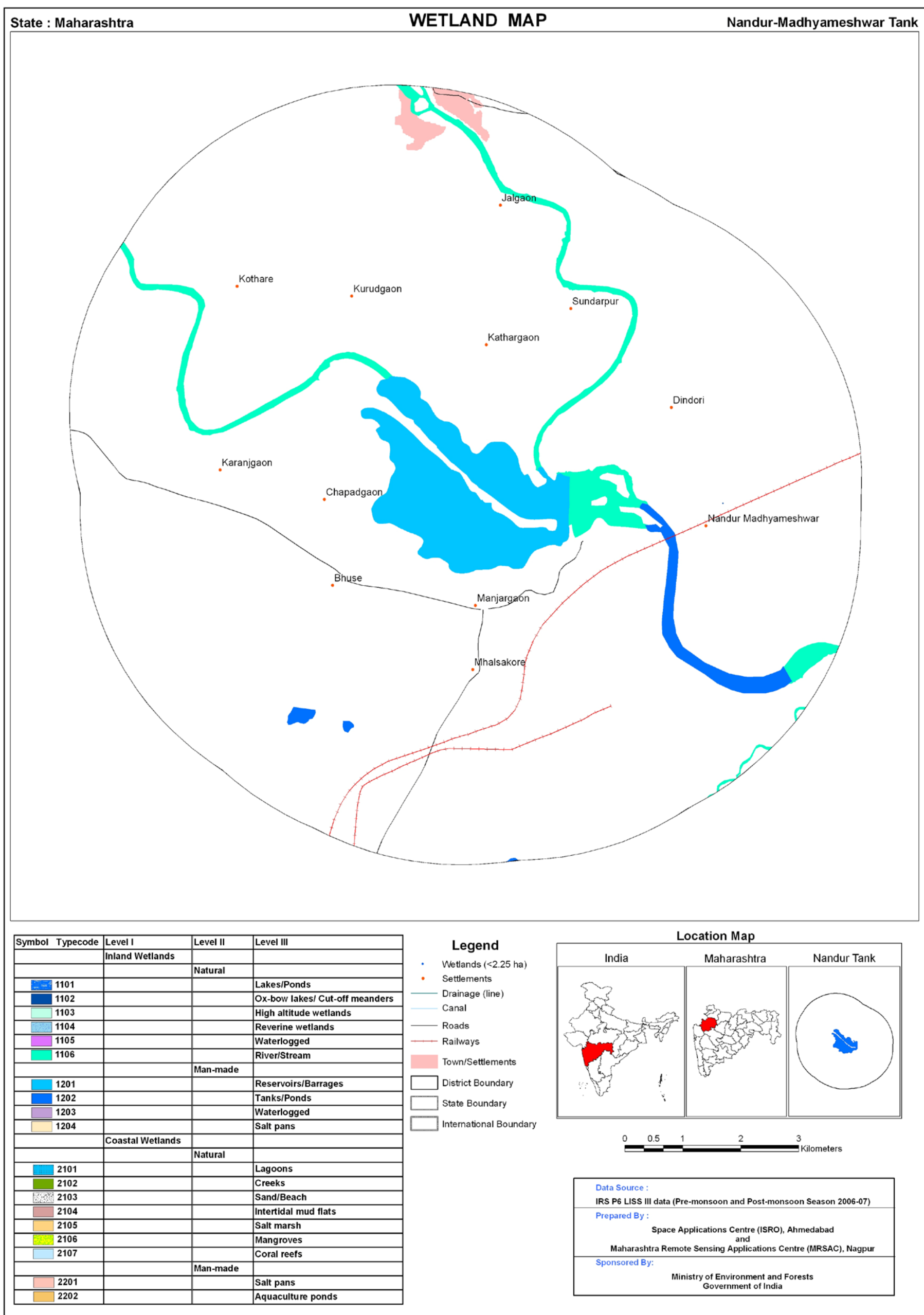
Plate 13: Wetland map - 5 km buffer area of Namdur Madhyameshwar Tank
