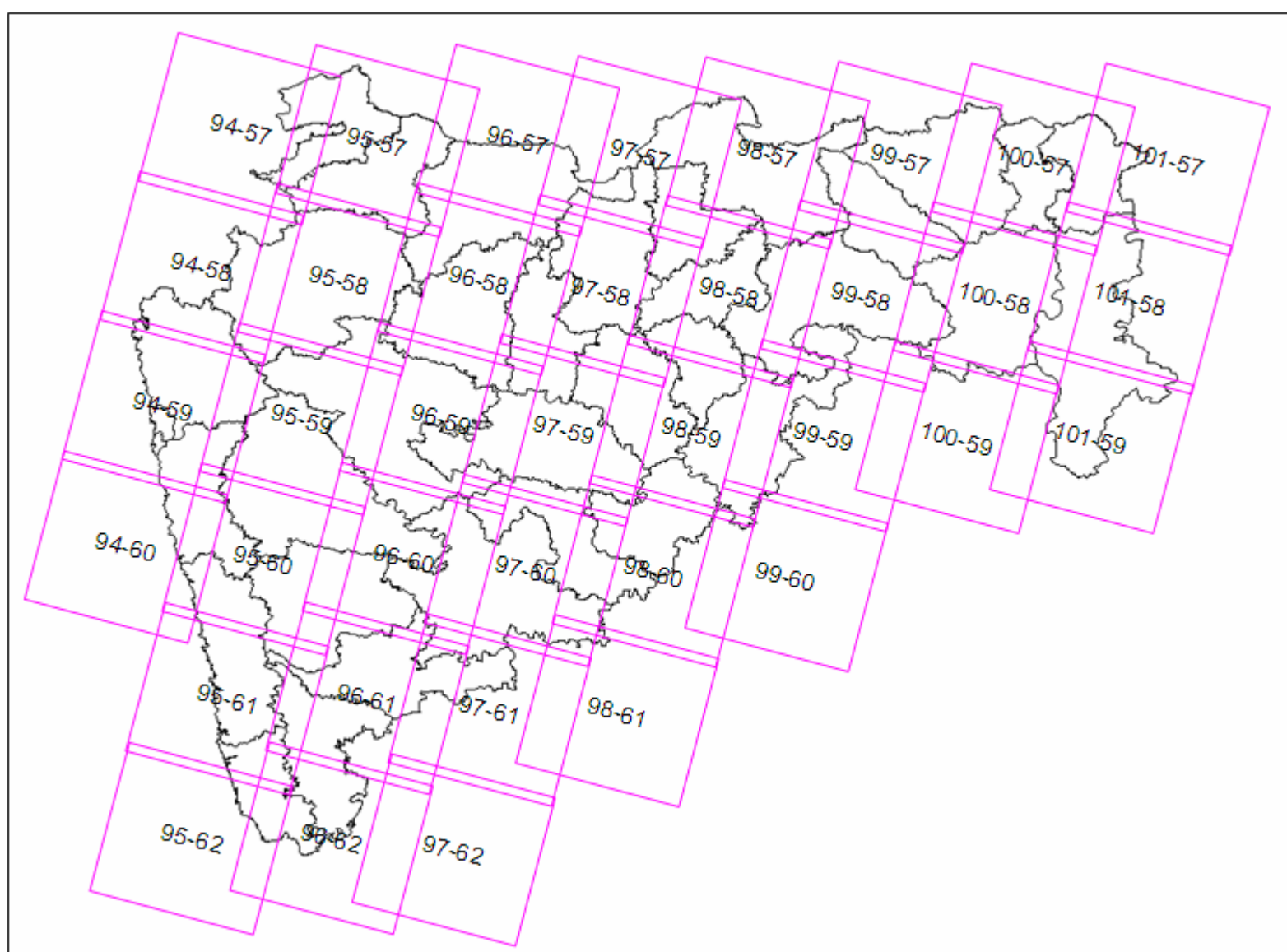
Figure 5: IRS P6 LISS-III coverage (path-row) of Maharashtra
