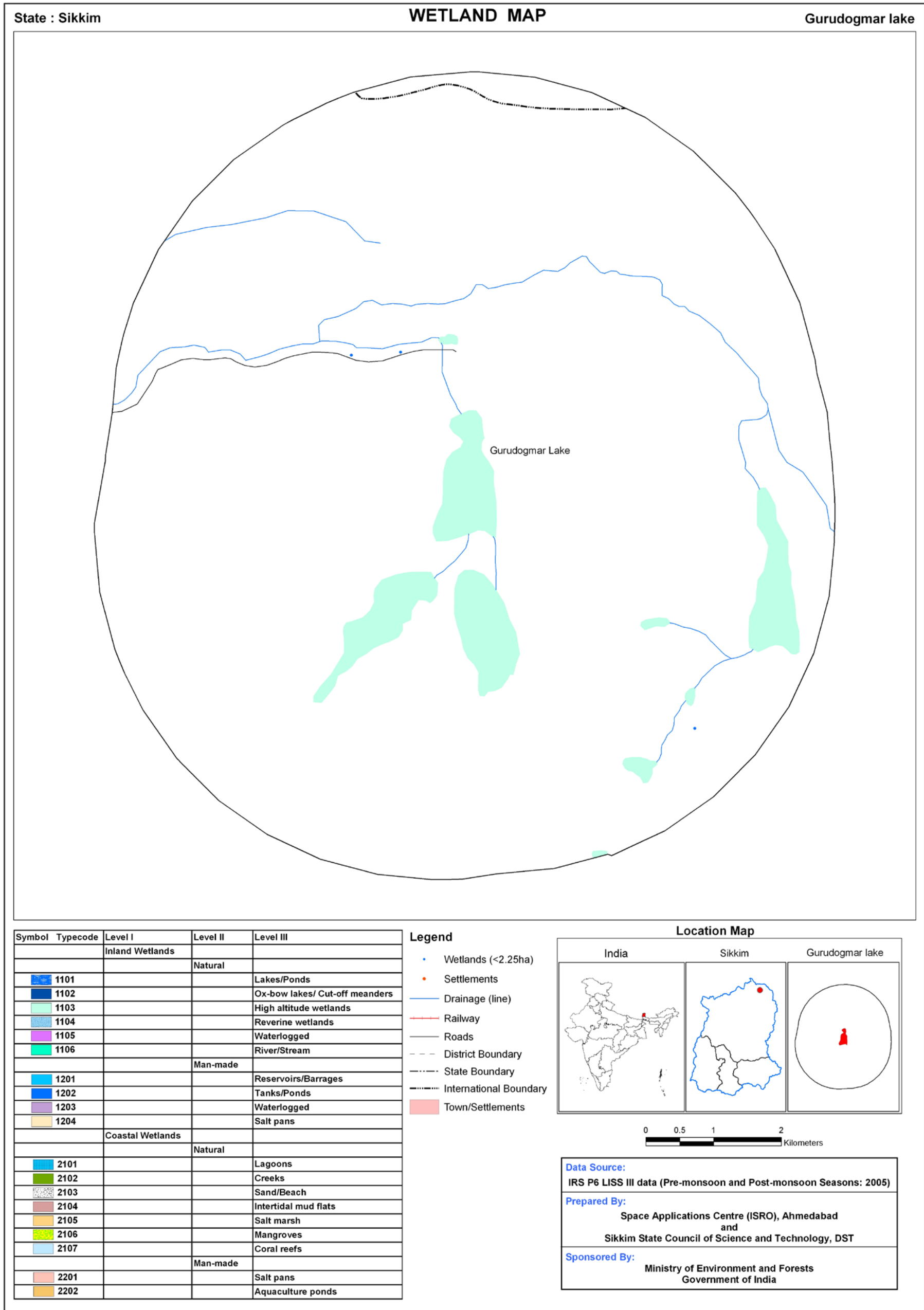
Plate 7: Wetland map - 5 km buffer area of Gurudogmar Lake
