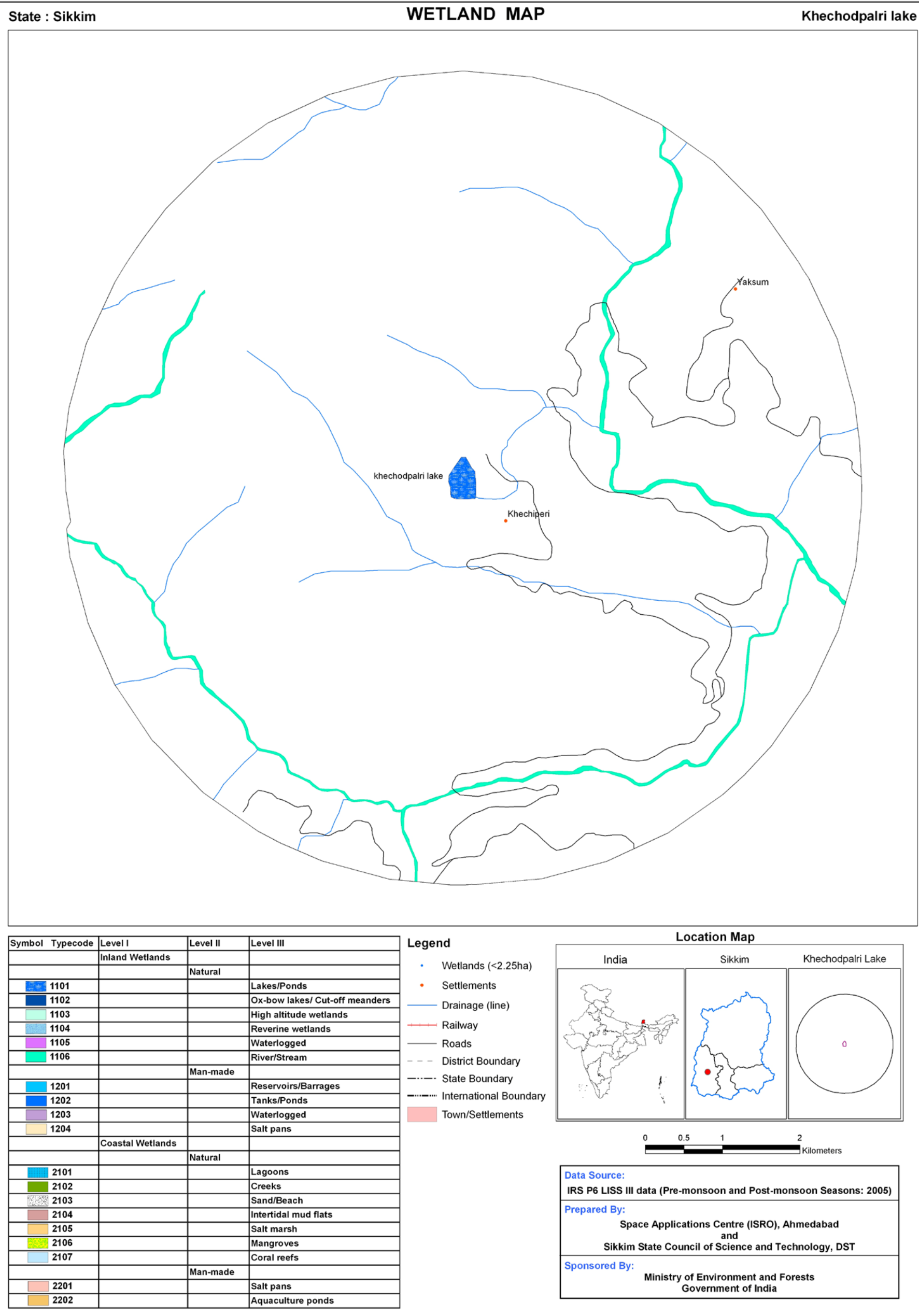
Plate 4: Wetland map - 5 km buffer area of Khechodpalri Lake
