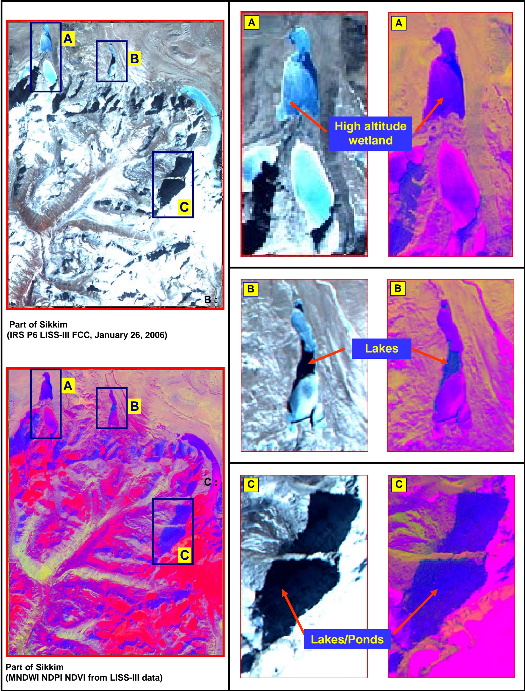
Plate 1: Major wetland types of Sikkim
